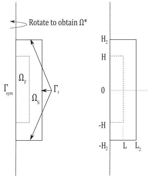
Fig. 1. Computational domain.
